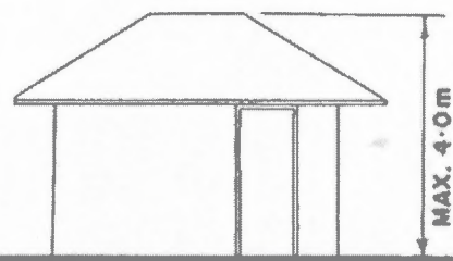
HIP OR COTTAGE ROOF
