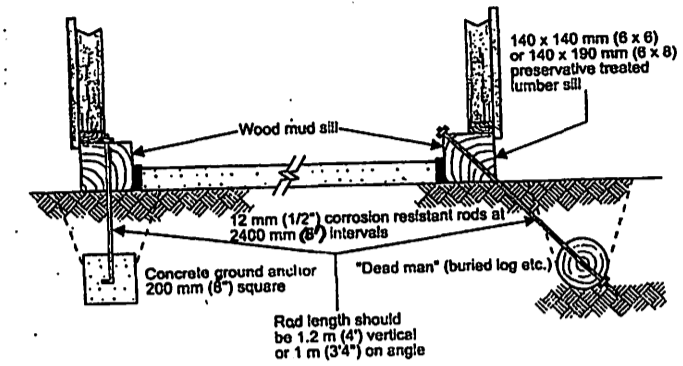
MUD SILL DETAIL (SMALL SHEDS)
