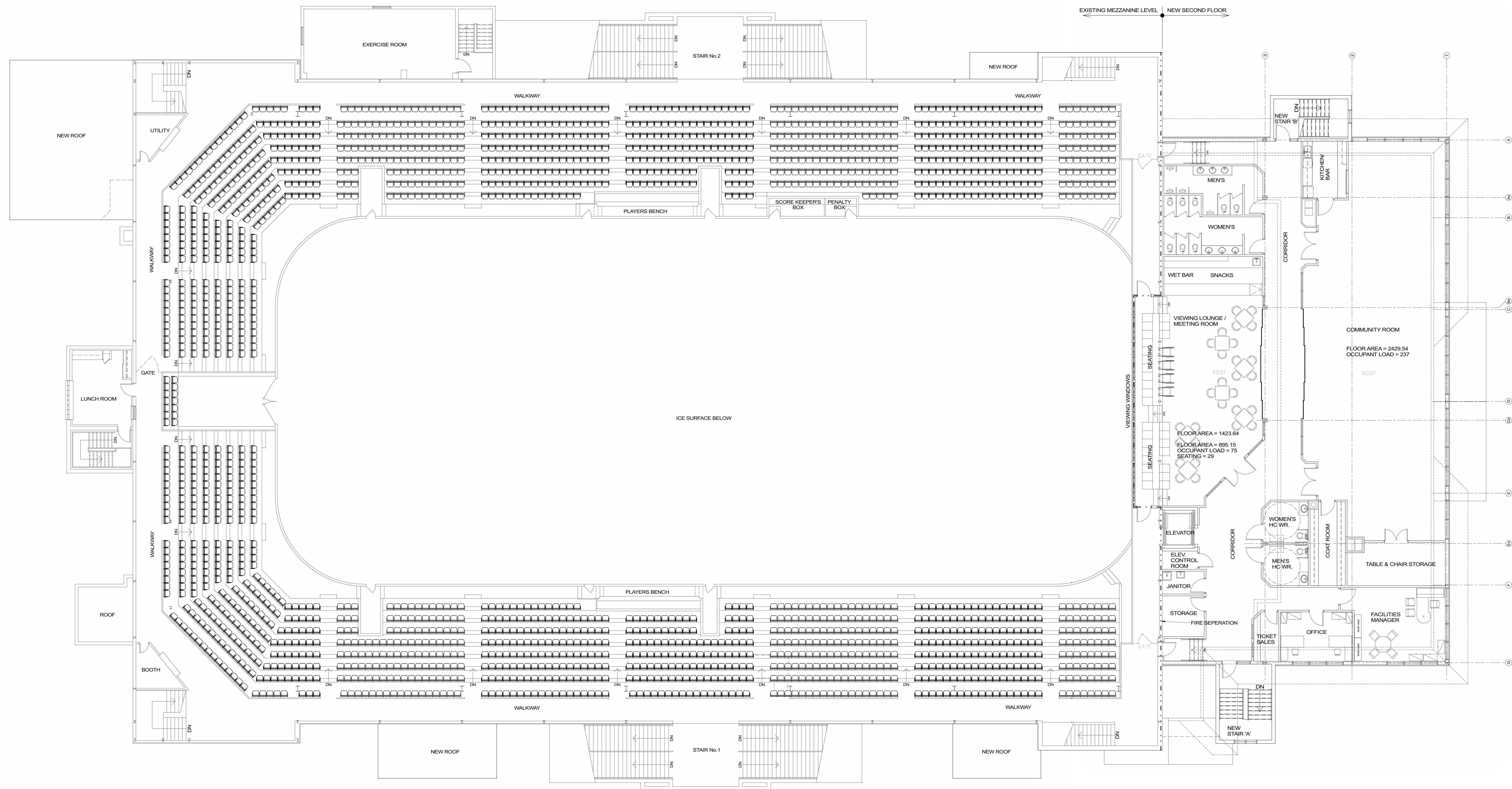
MEZZANINE / SECOND FLOOR PLAN 3/32" = 1'-0"
